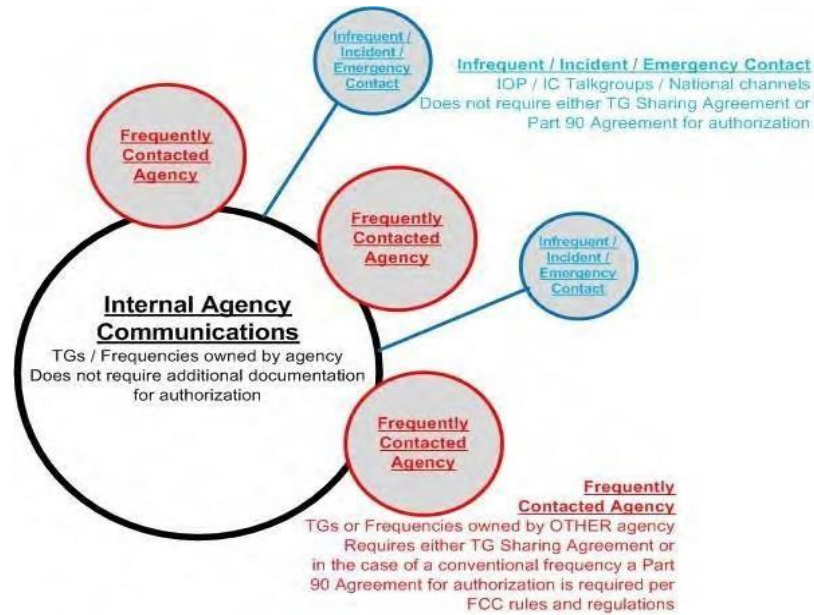
Figure 1 - Generic Talkgroup
