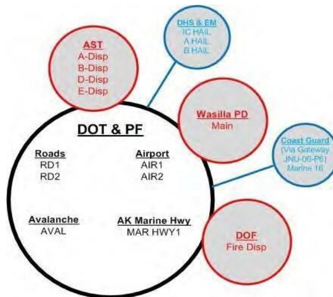
Figure 1 - Generic Talkgroup
